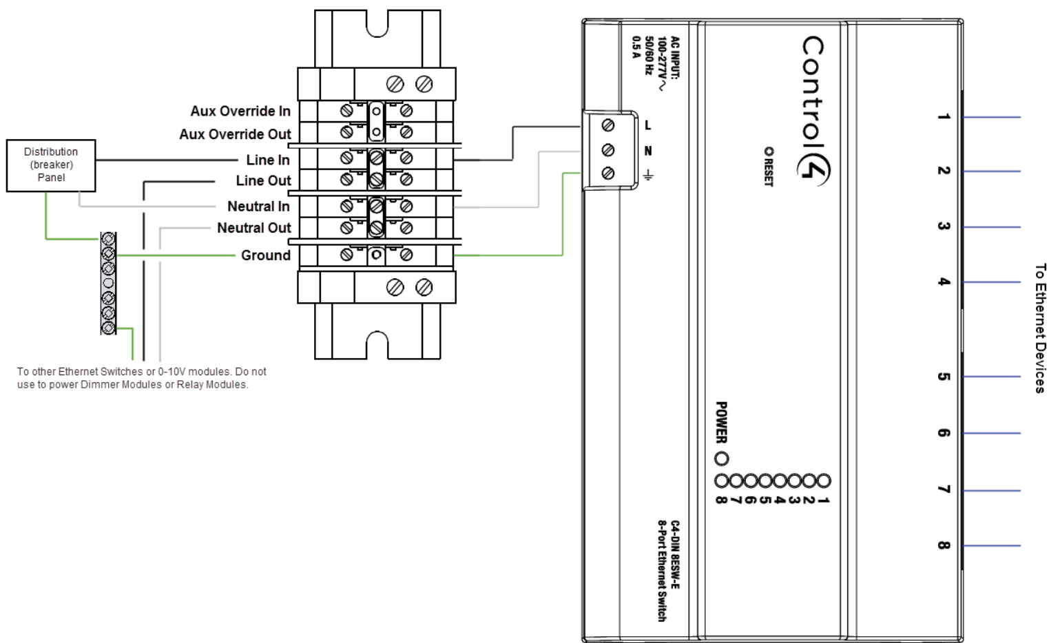
Figure 2. 8-Port Ethernet Switch Terminal Block Wiring
