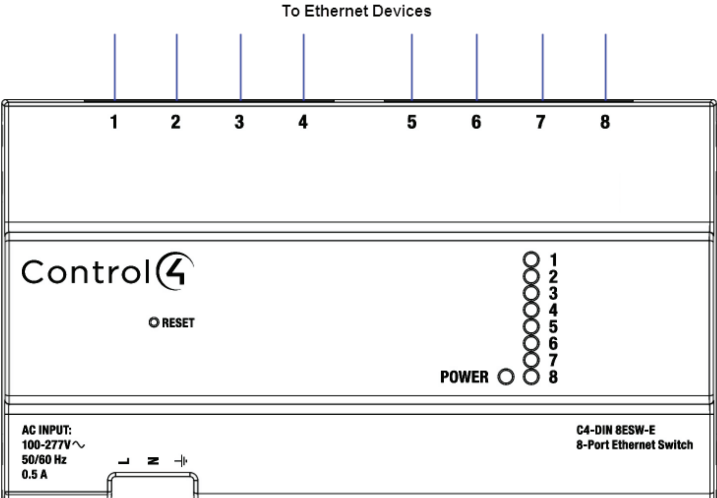
Figure 1. 8-Port Ethernet Switch Wiring Diagram
