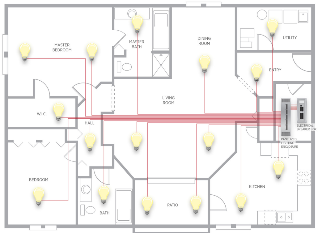
Figure 3. Centralized Panel Design Example
