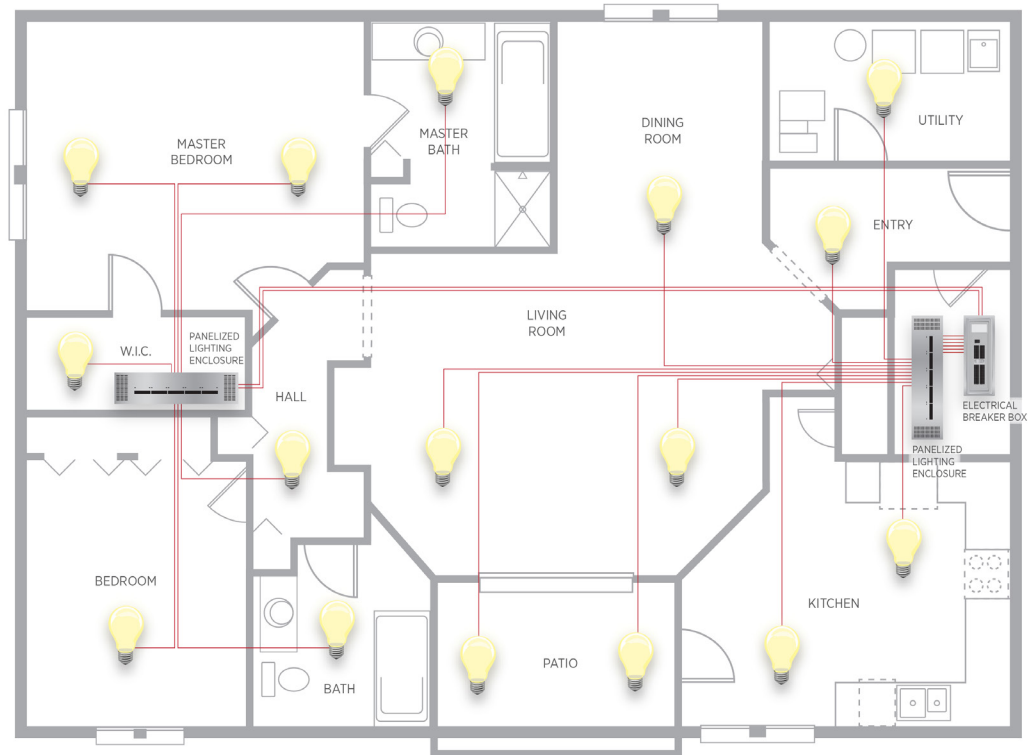
Figure 4. Distributed Panel Design Example
